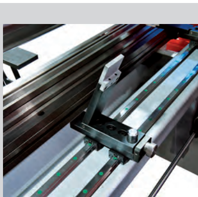
Flip up type back gauge micro adjustment fingers
